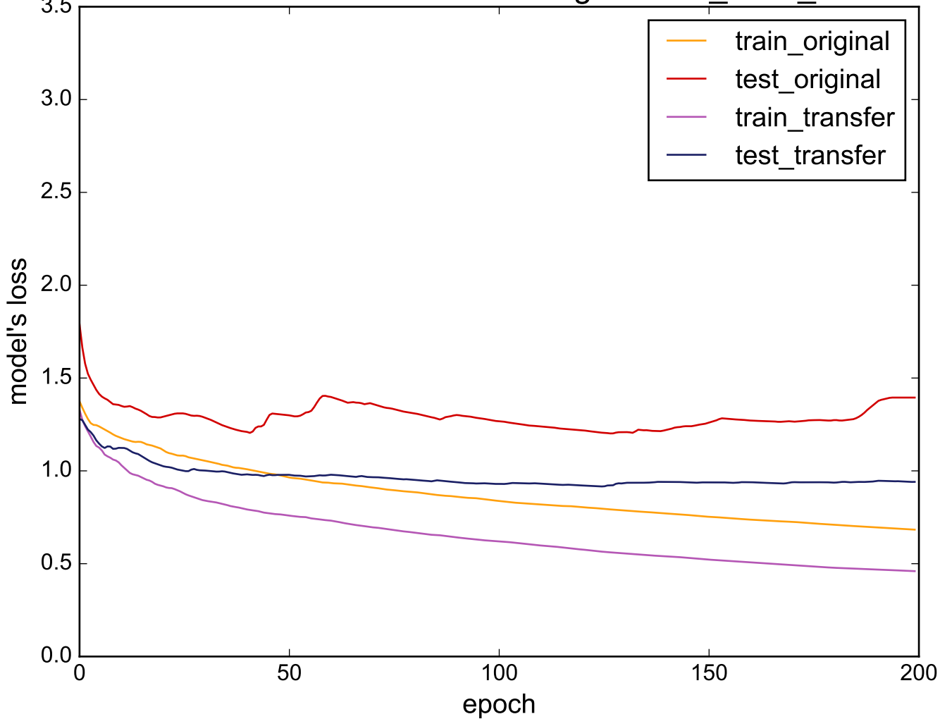
Source: MiddlePhalanxTW - Target: CinC_ECG_torso
