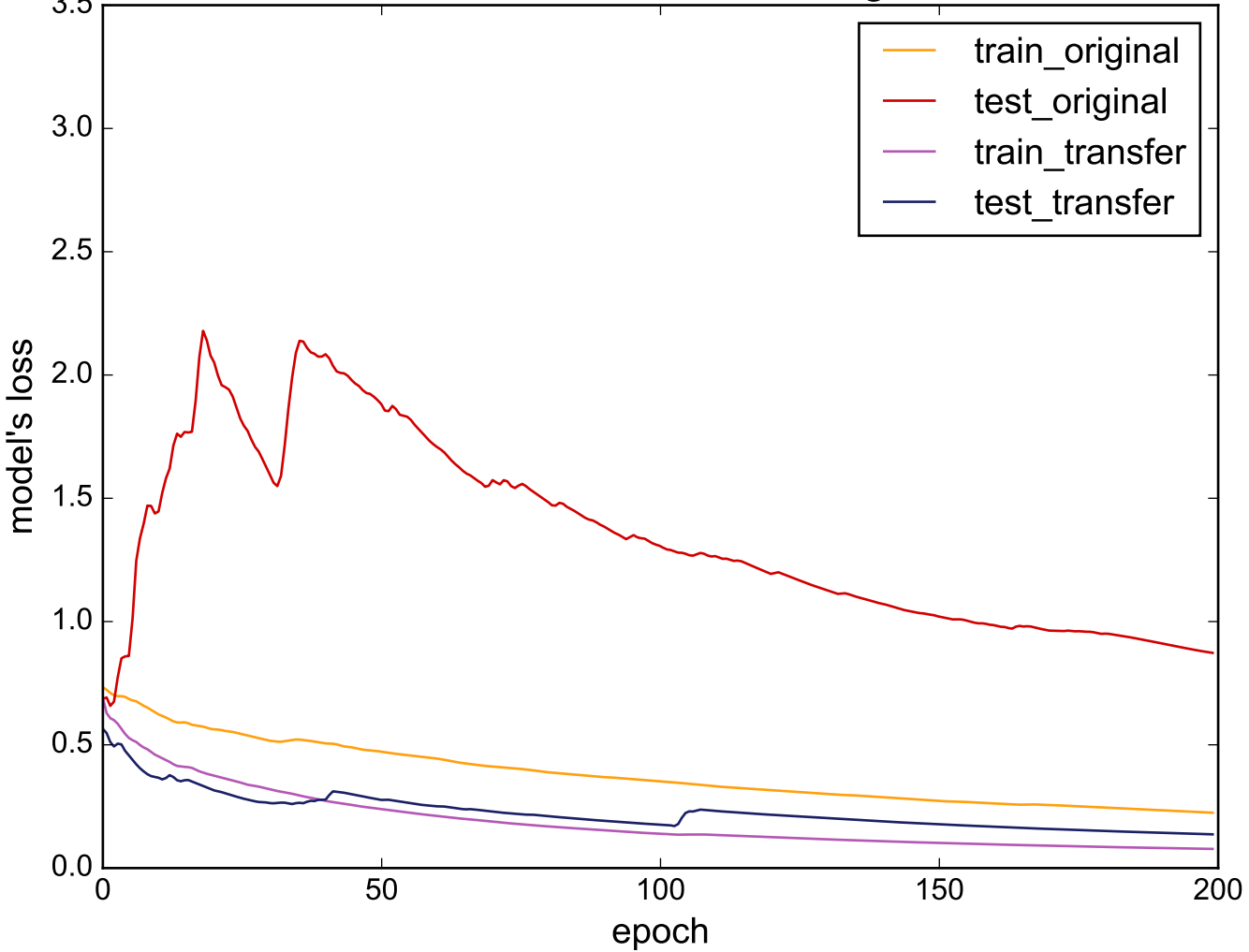
Source: MiddlePhalanxTW - Target: Coffee
