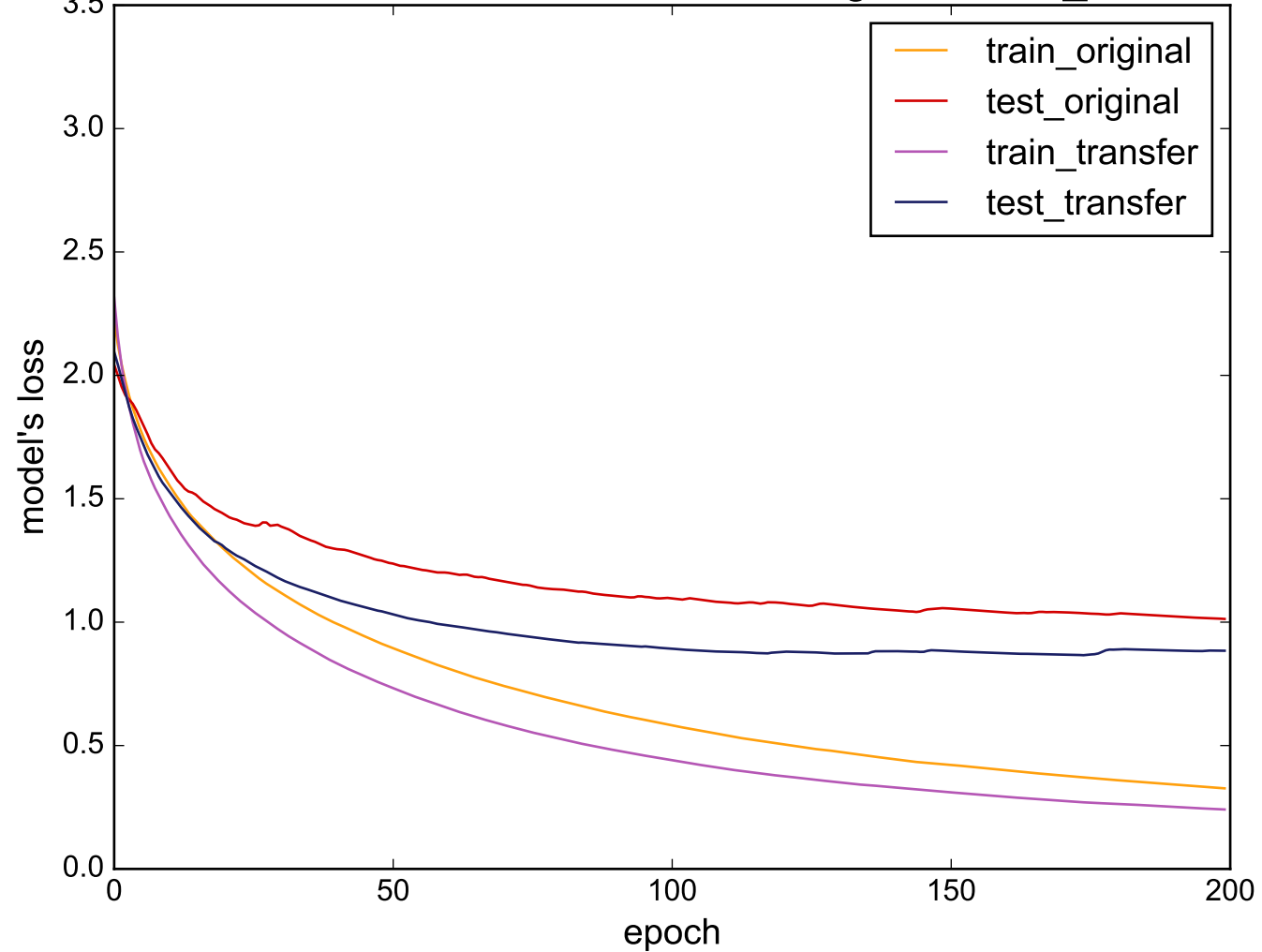
Source: MiddlePhalanxTW - Target: Cricket_X
