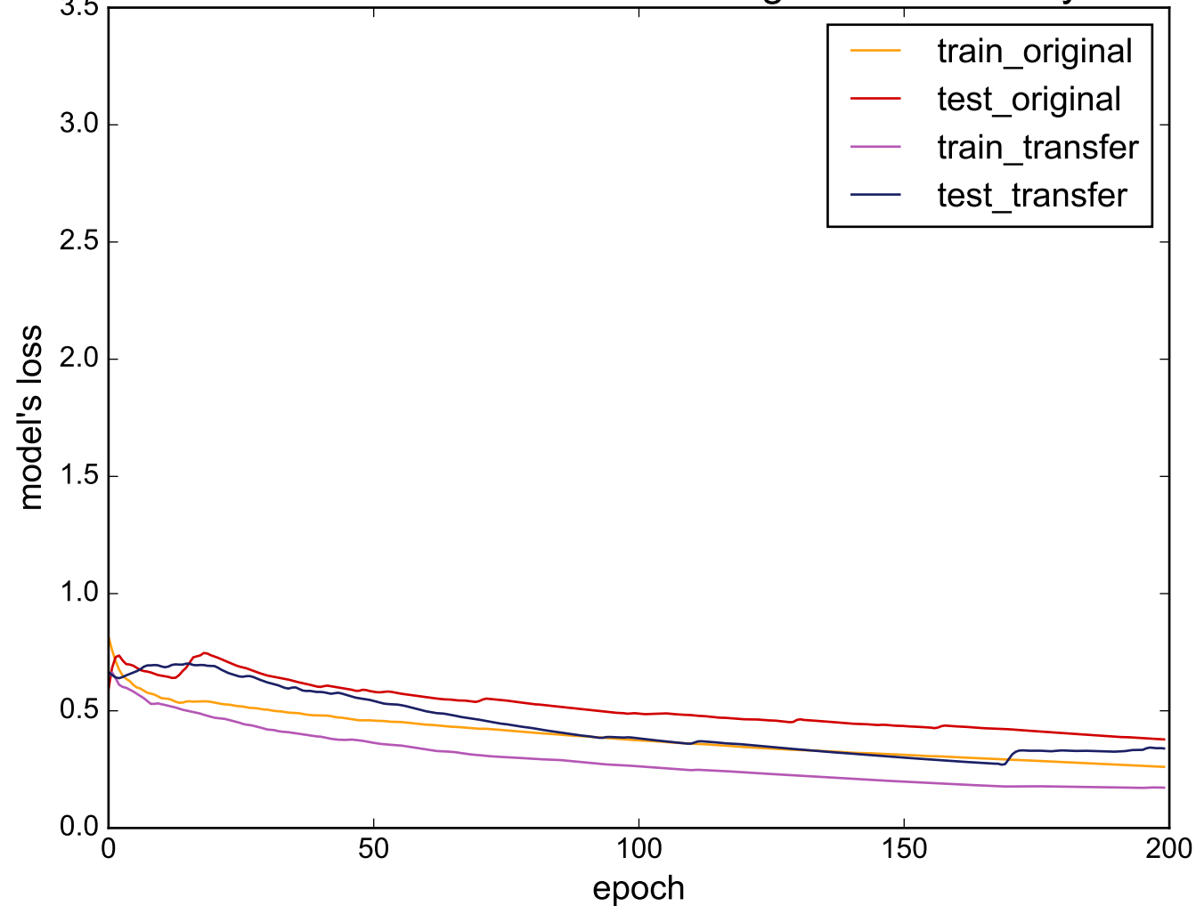
Source: MiddlePhalanxTW - Target: ECGFiveDays
