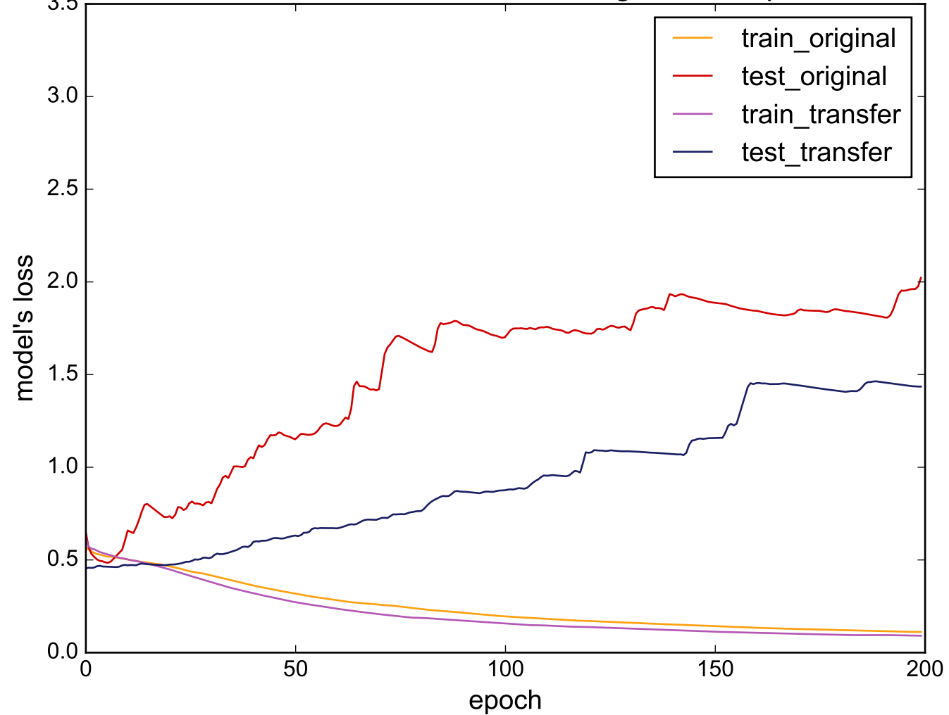
Source: MiddlePhalanxTW - Target: Earthquakes
