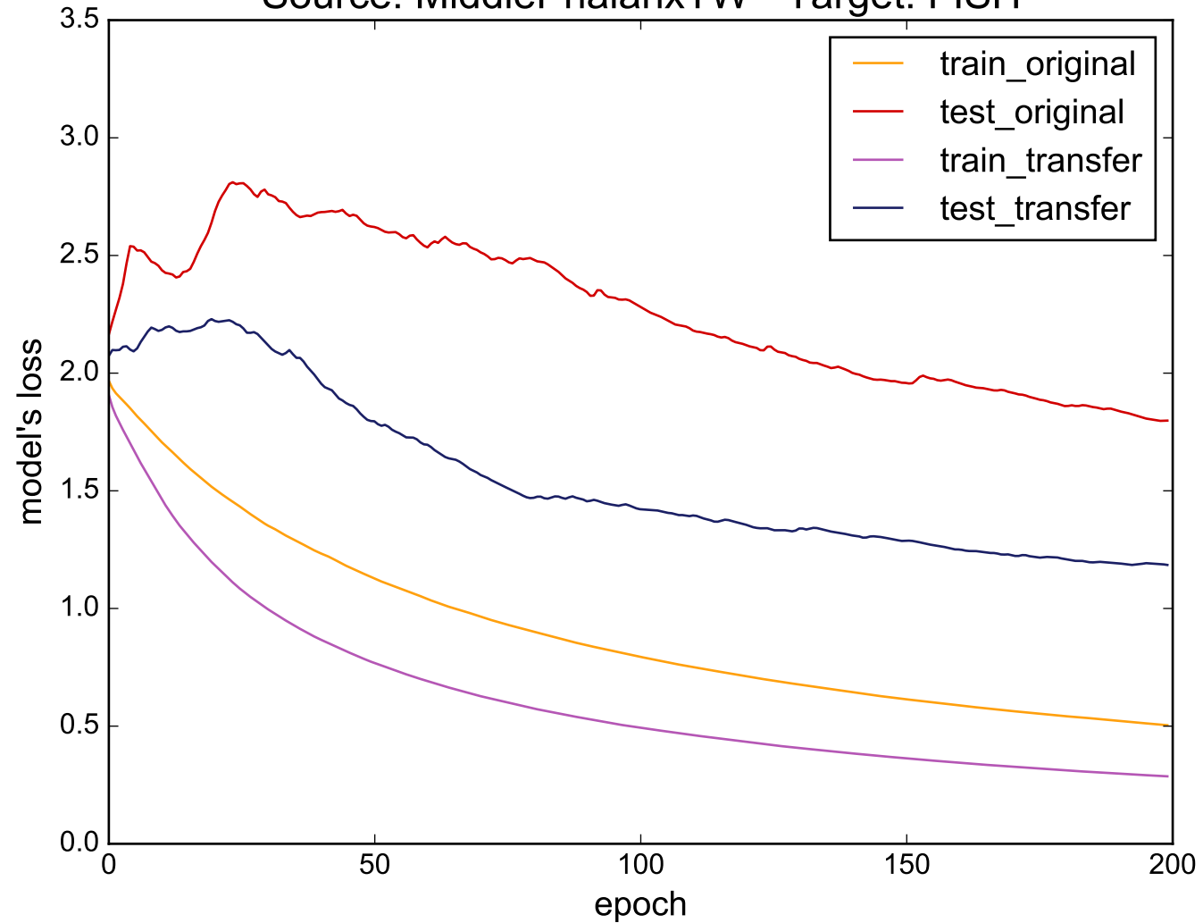
Source: MiddlePhalanxTW - Target: FISH
