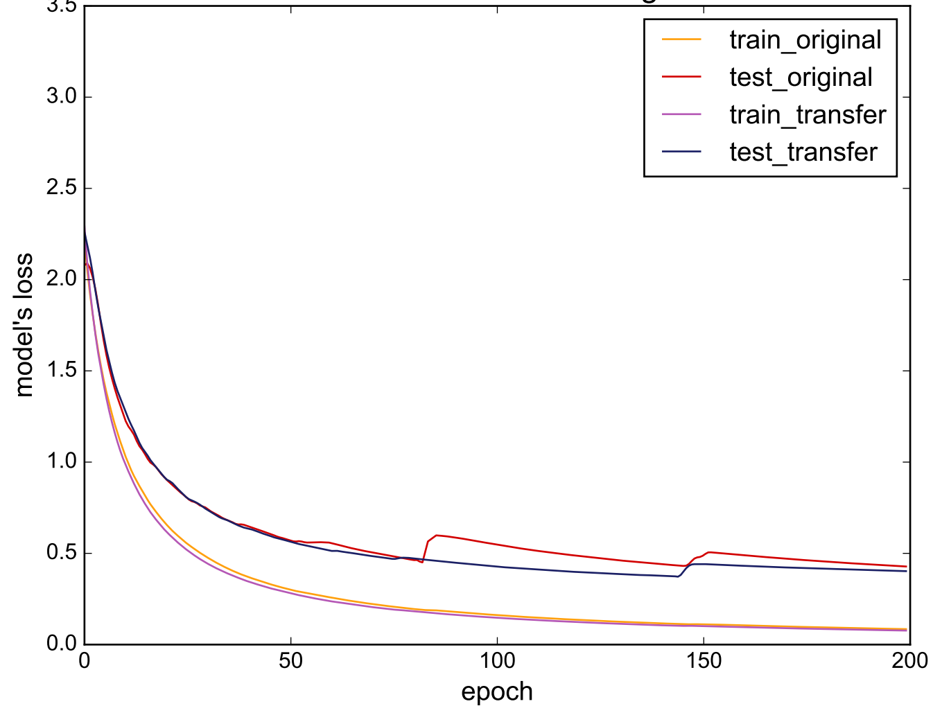
Source: MiddlePhalanxTW - Target: FaceAll
