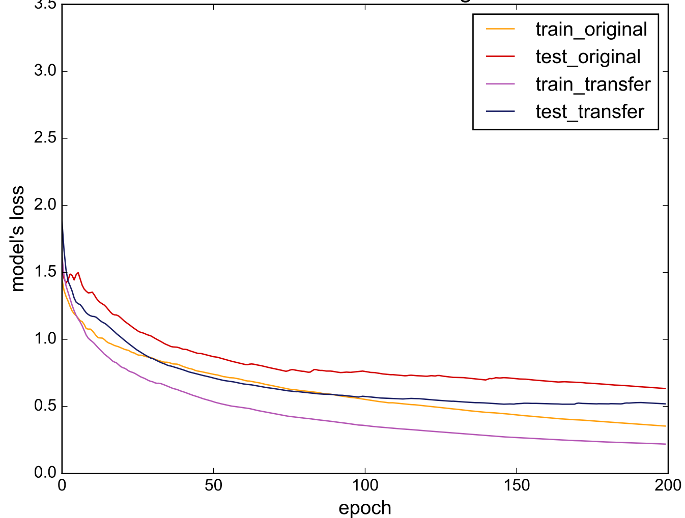
Source: MiddlePhalanxTW - Target: FaceFour
