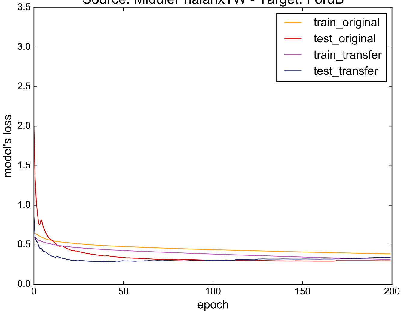
Source: MiddlePhalanxTW - Target: FordB
