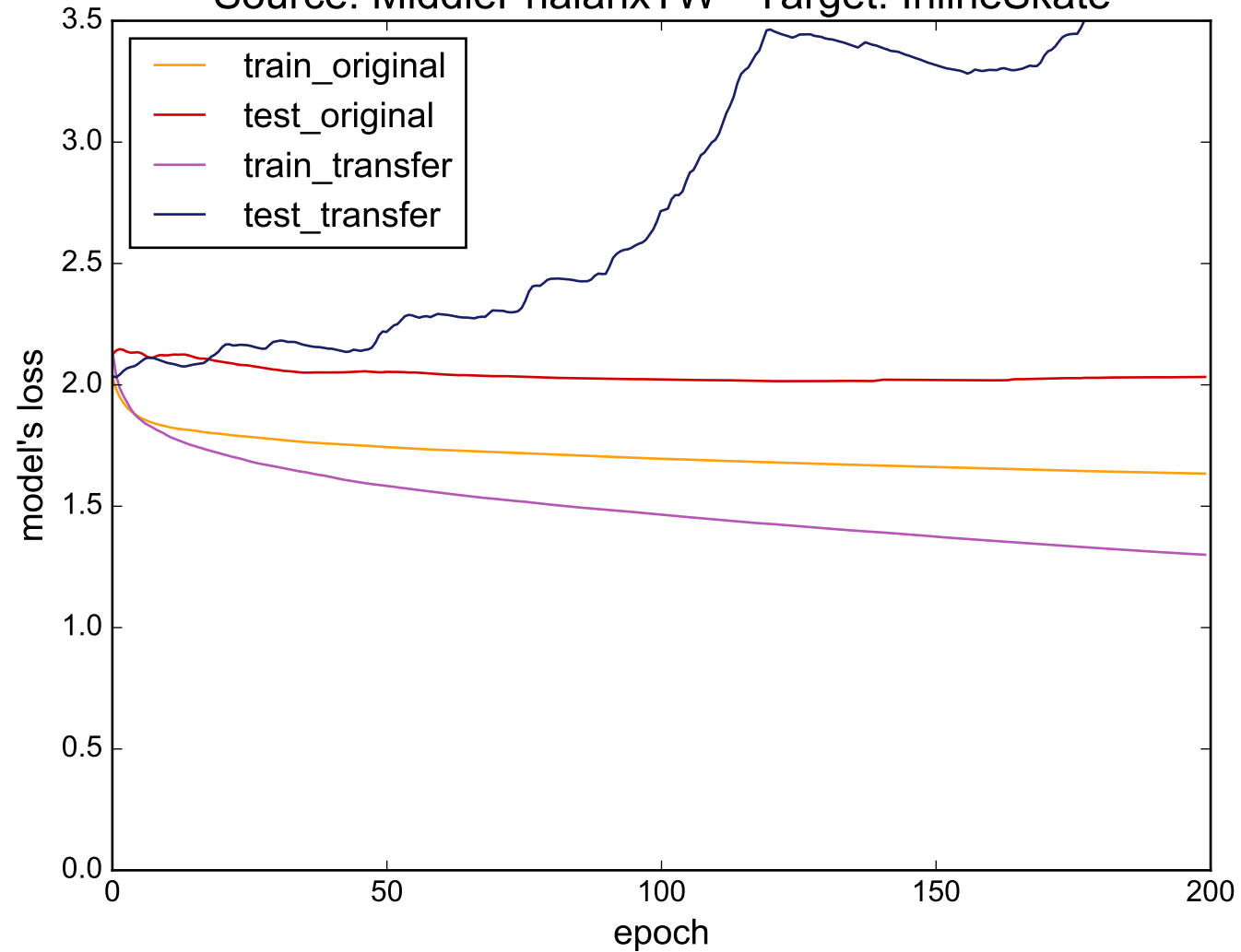
Source: MiddlePhalanxTW - Target: InlineSkate
