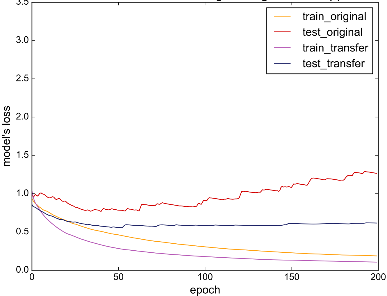
Source: MiddlePhalanxTW - Target: LargeKitchenAppliances
