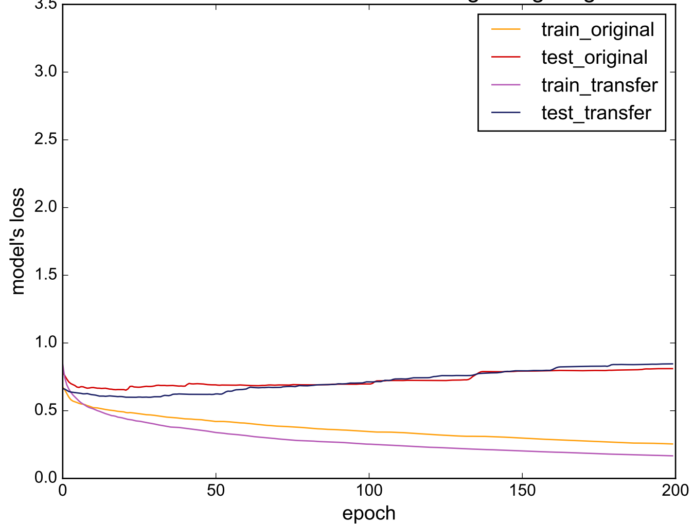
Source: MiddlePhalanxTW - Target: Lighting2
