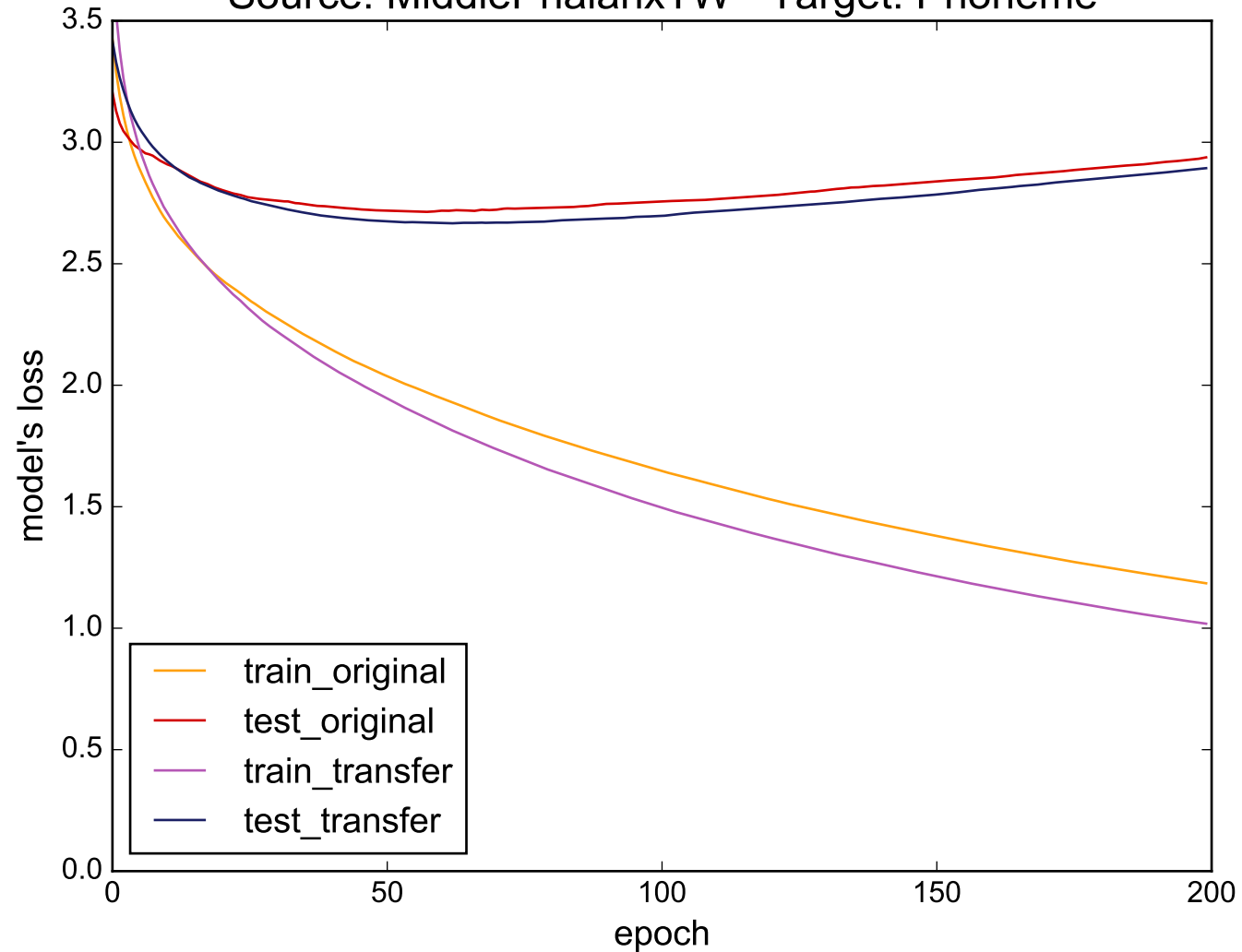
Source: MiddlePhalanxTW - Target: Phoneme
