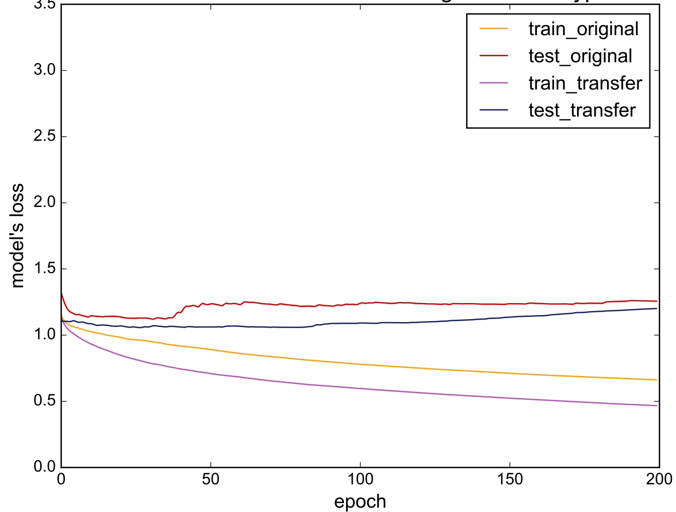
Source: MiddlePhalanxTW - Target: ScreenType
