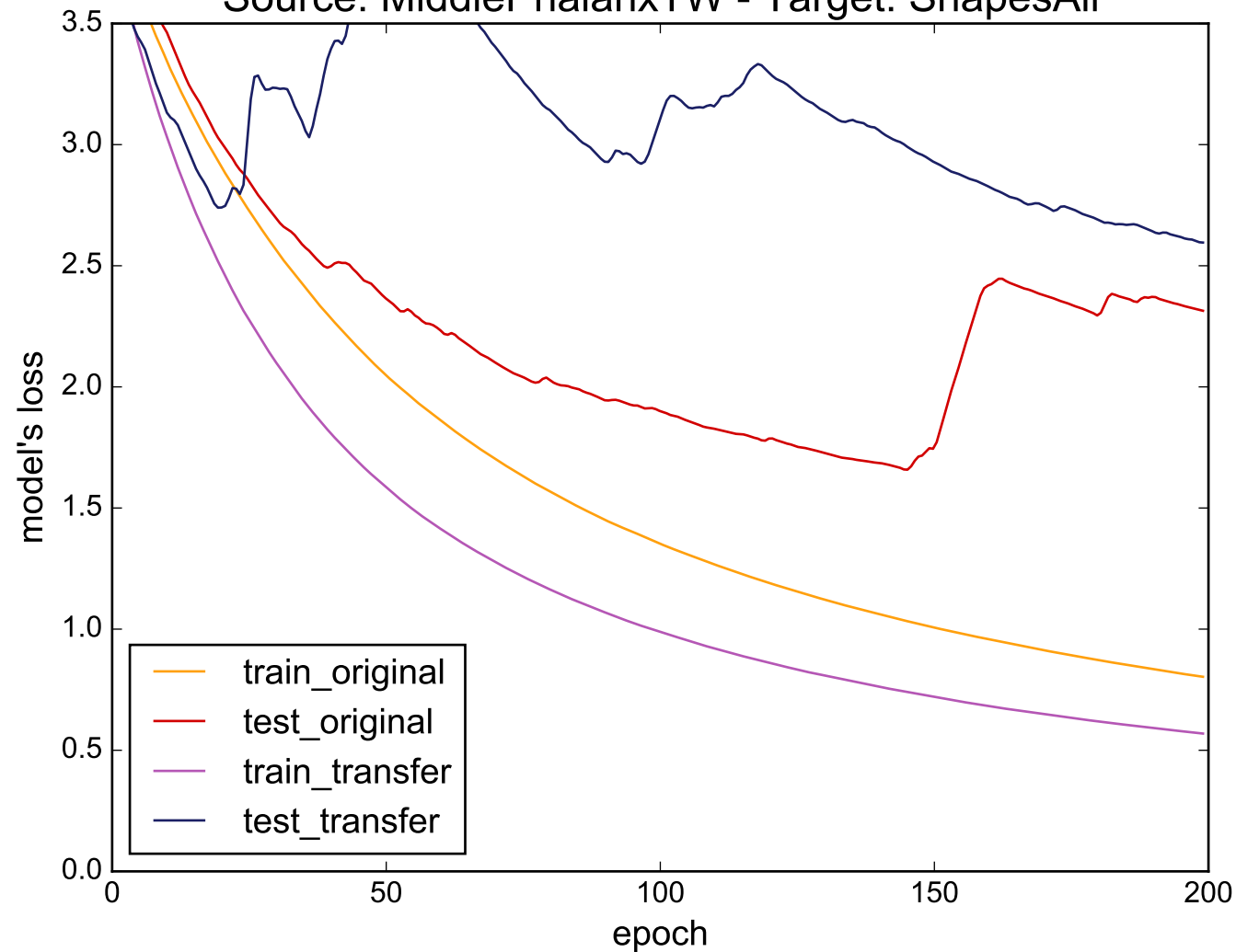
Source: MiddlePhalanxTW - Target: ShapesAll
