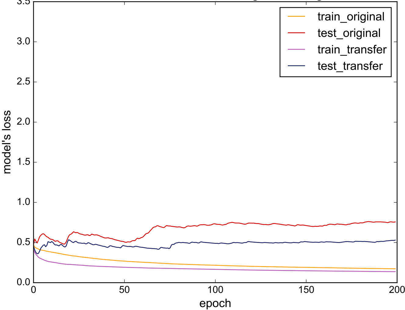
Source: MiddlePhalanxTW - Target: StarLightCurves
