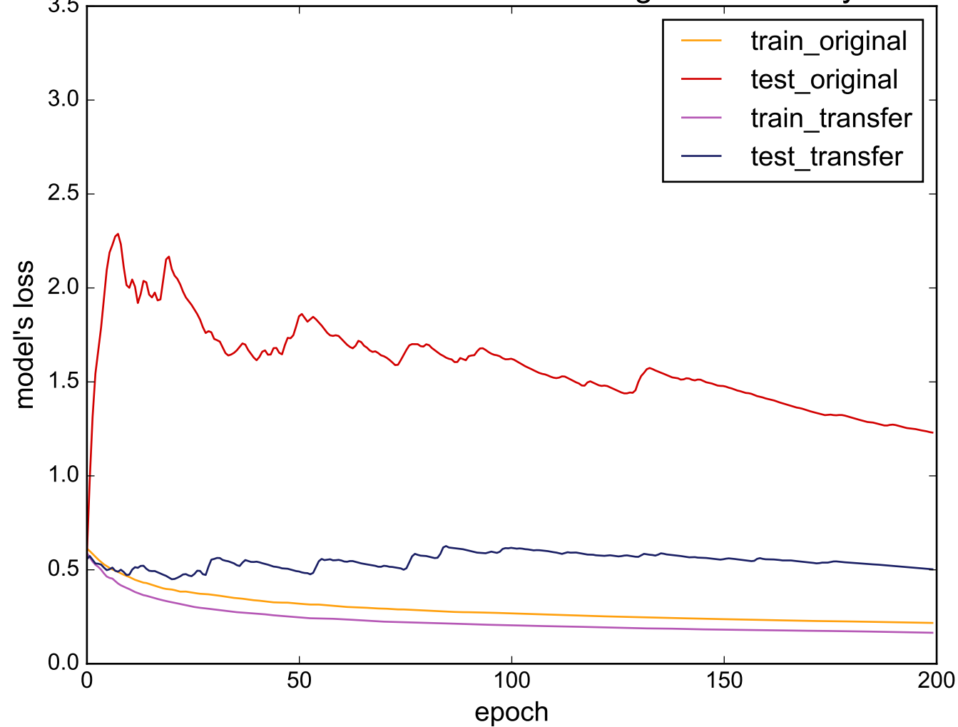
Source: MiddlePhalanxTW - Target: Strawberry
