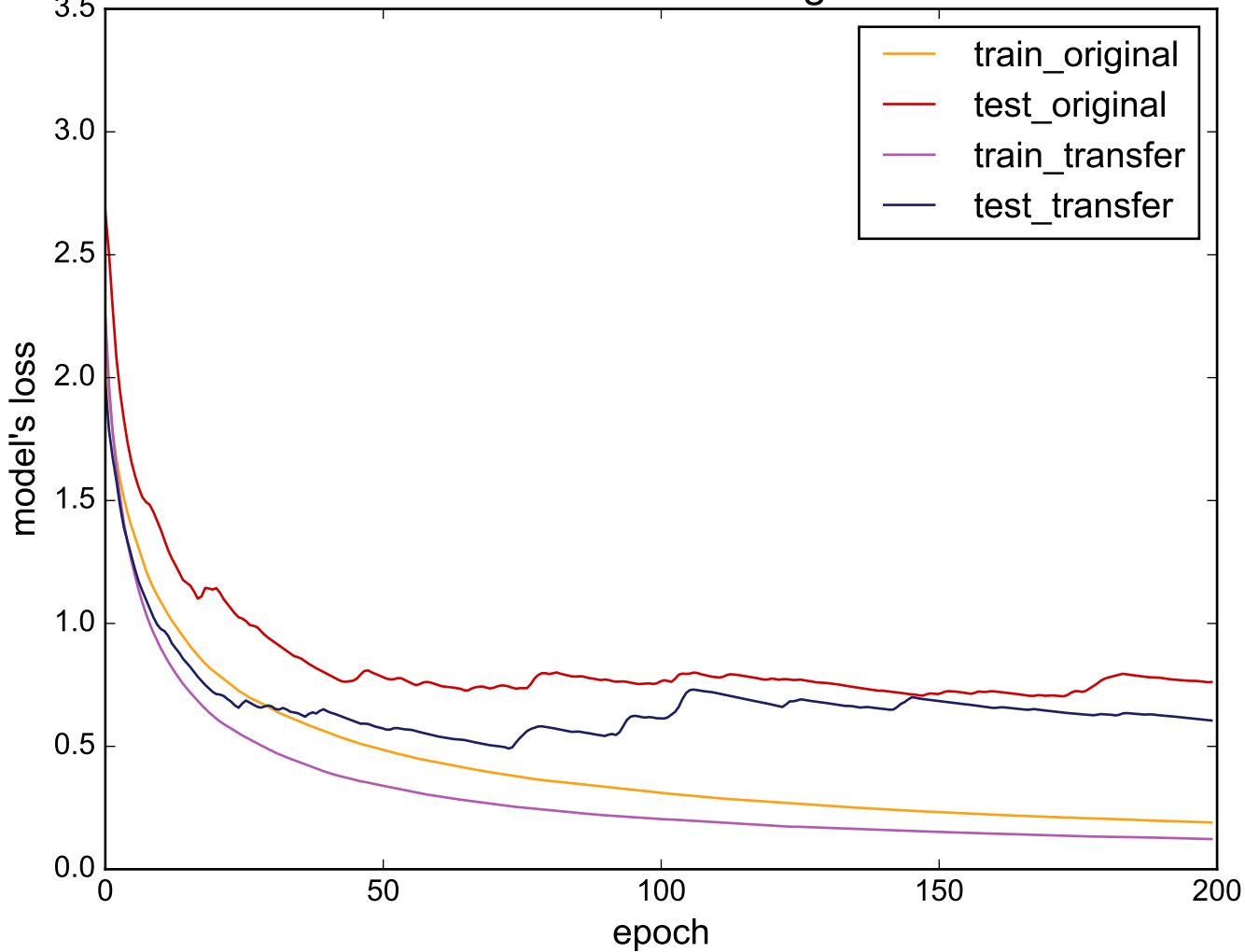
Source: MiddlePhalanxTW - Target: SwedishLeaf
