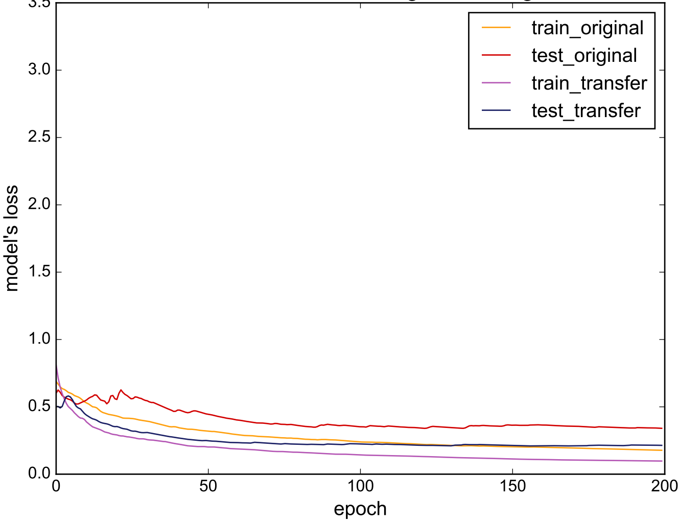
Source: MiddlePhalanxTW - Target: ToeSegmentation1
