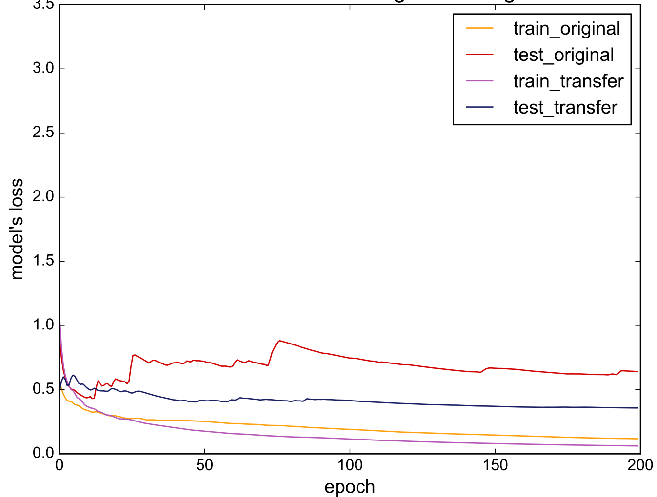
Source: MiddlePhalanxTW - Target: ToeSegmentation2
