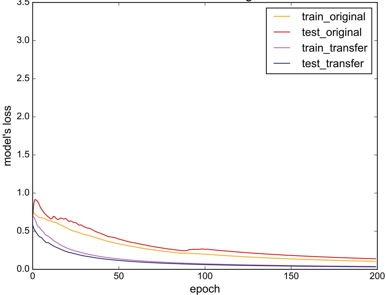
Source: MiddlePhalanxTW - Target: TwoLeadECG
