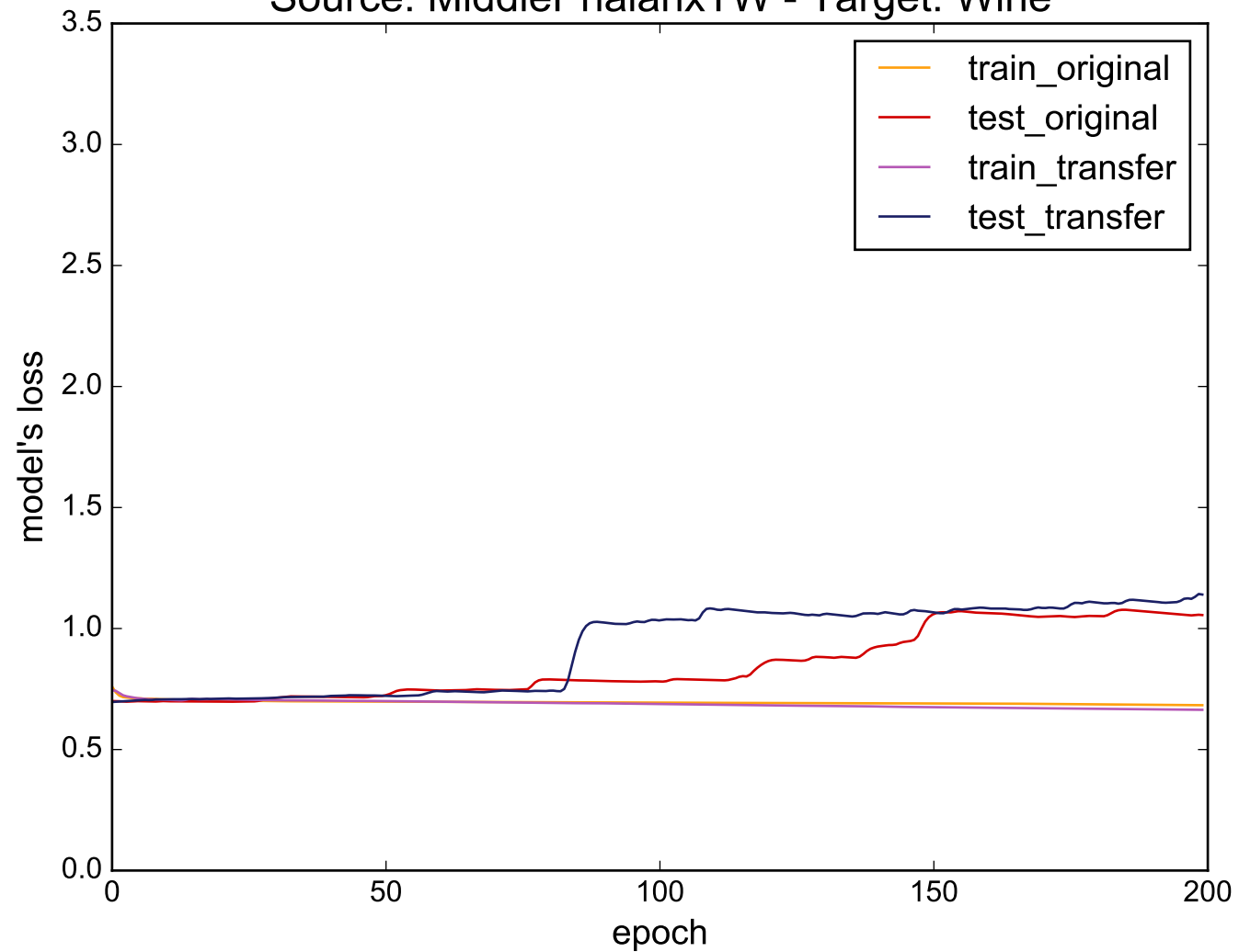
Source: MiddlePhalanxTW - Target: Wine
