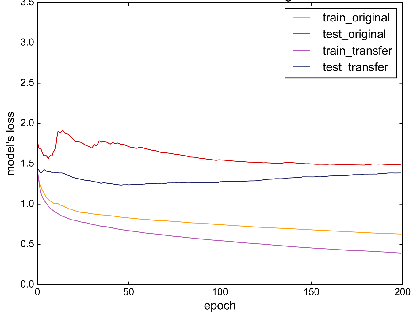
Source: MiddlePhalanxTW - Target: Worms
