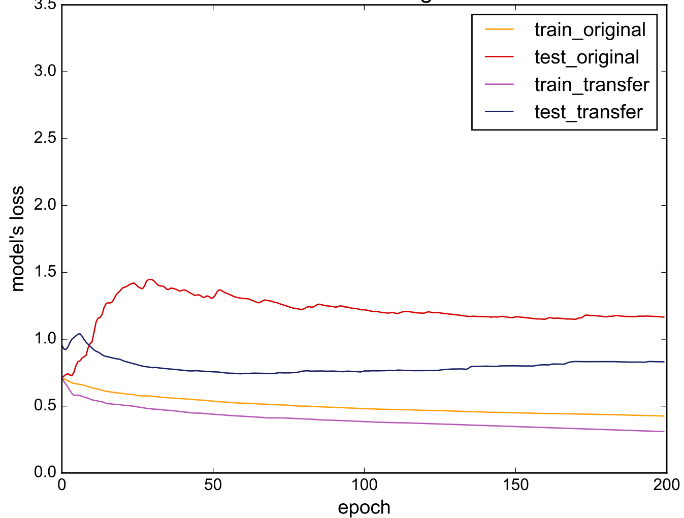
Source: MiddlePhalanxTW - Target: WormsTwoClass
