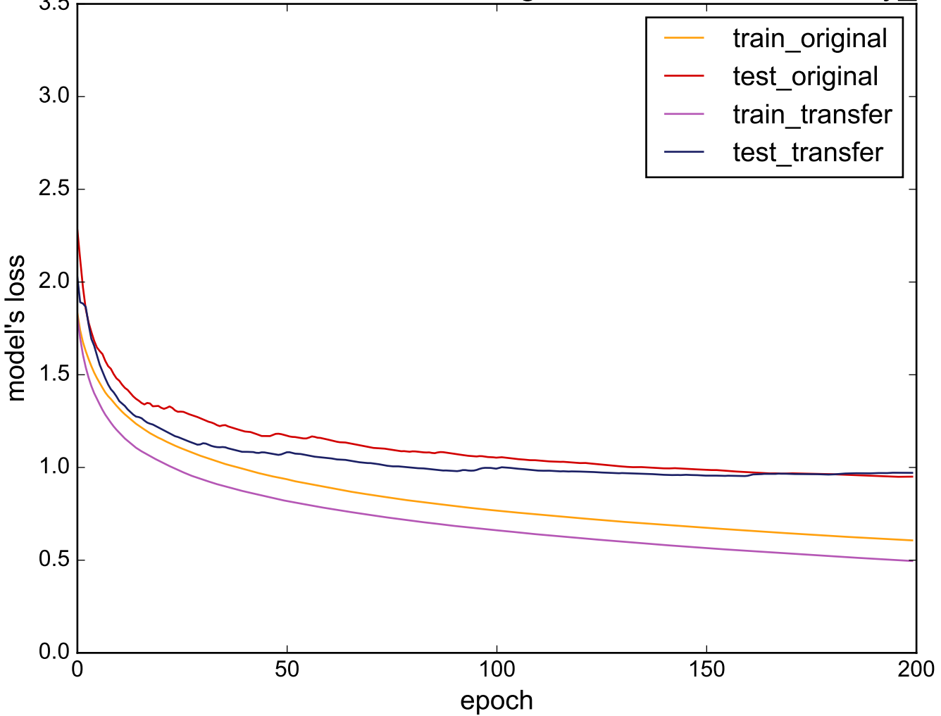
Source: MiddlePhalanxTW - Target: uWaveGestureLibrary_X
