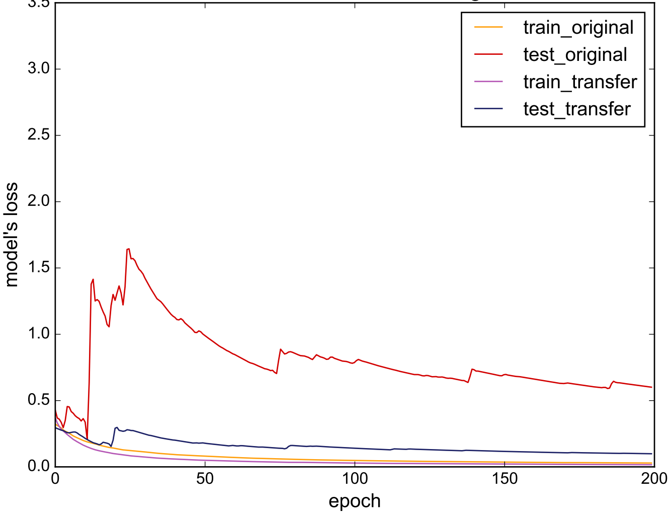
Source: MiddlePhalanxTW - Target: wafer
