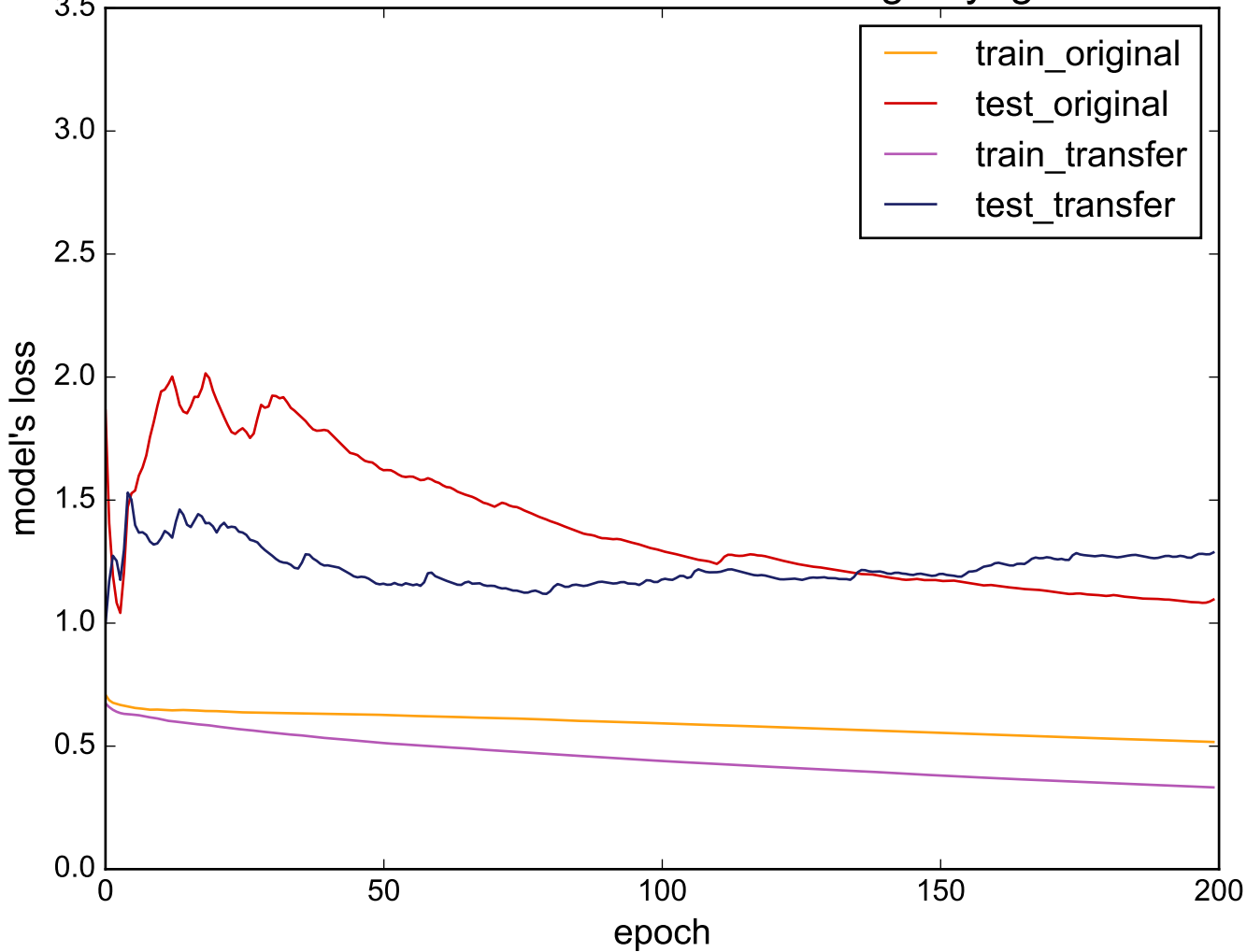
Source: MiddlePhalanxTW - Target: yoga
