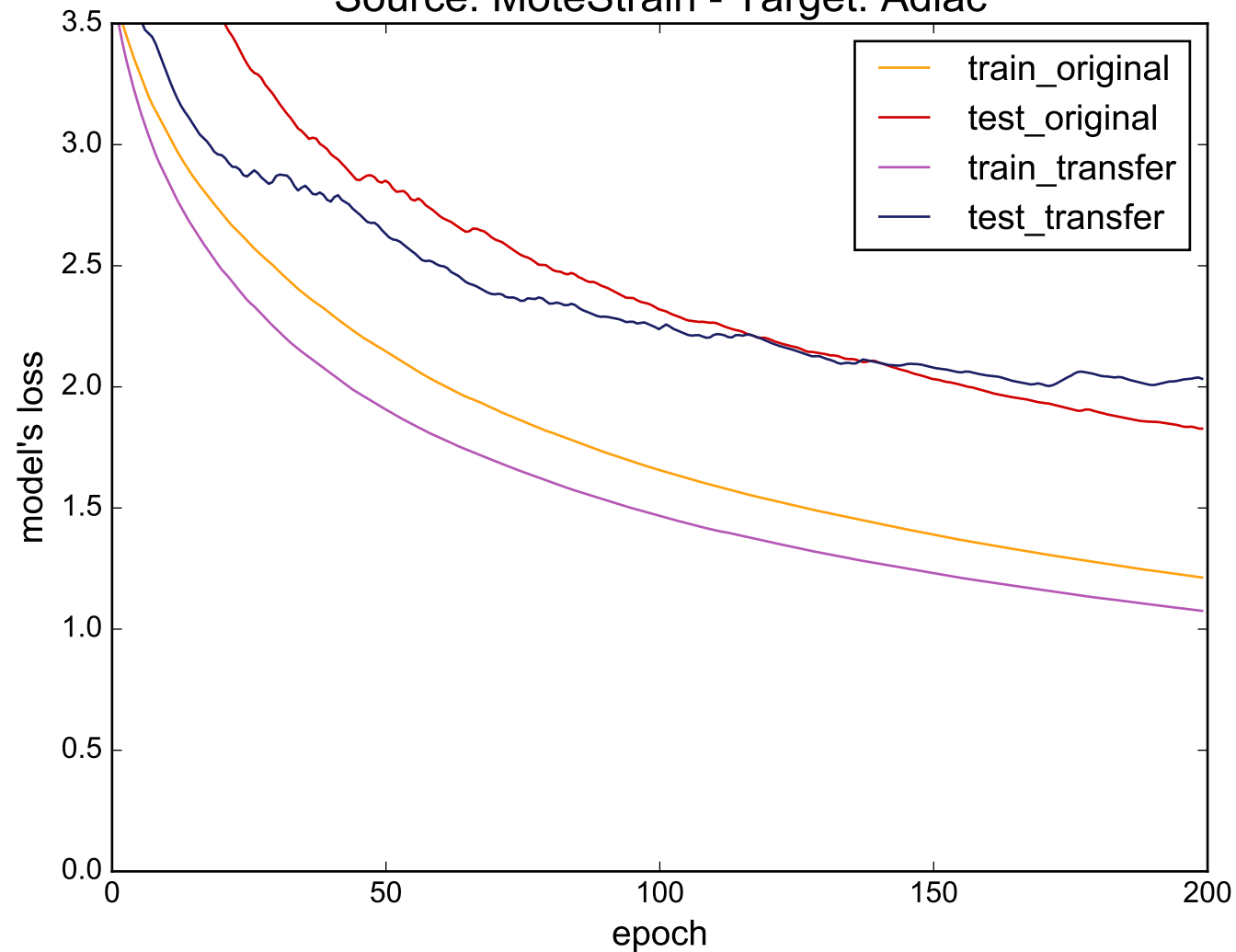
Source: MoteStrain - Target: Adiac
