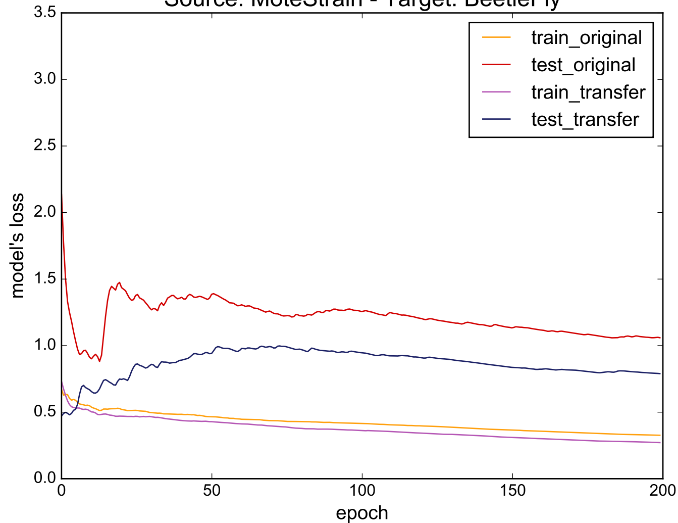
Source: MoteStrain - Target: BeetleFly
