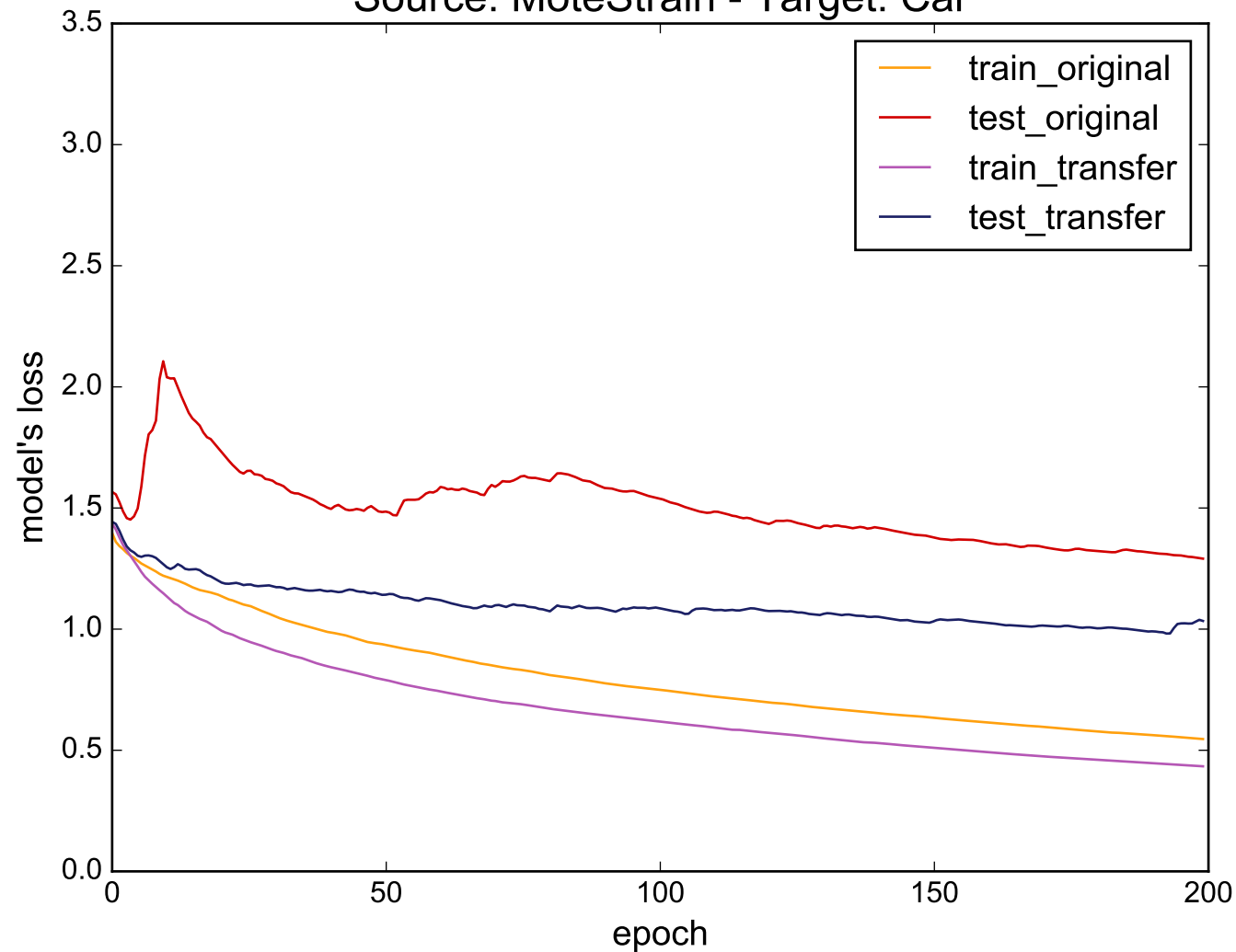
Source: MoteStrain - Target: Car
