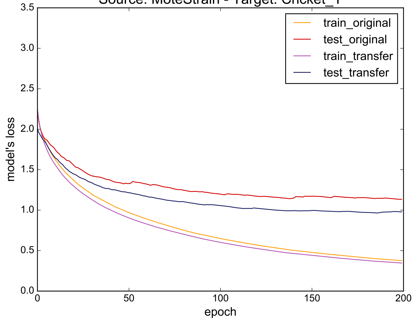
Source: MoteStrain - Target: Cricket_Y
