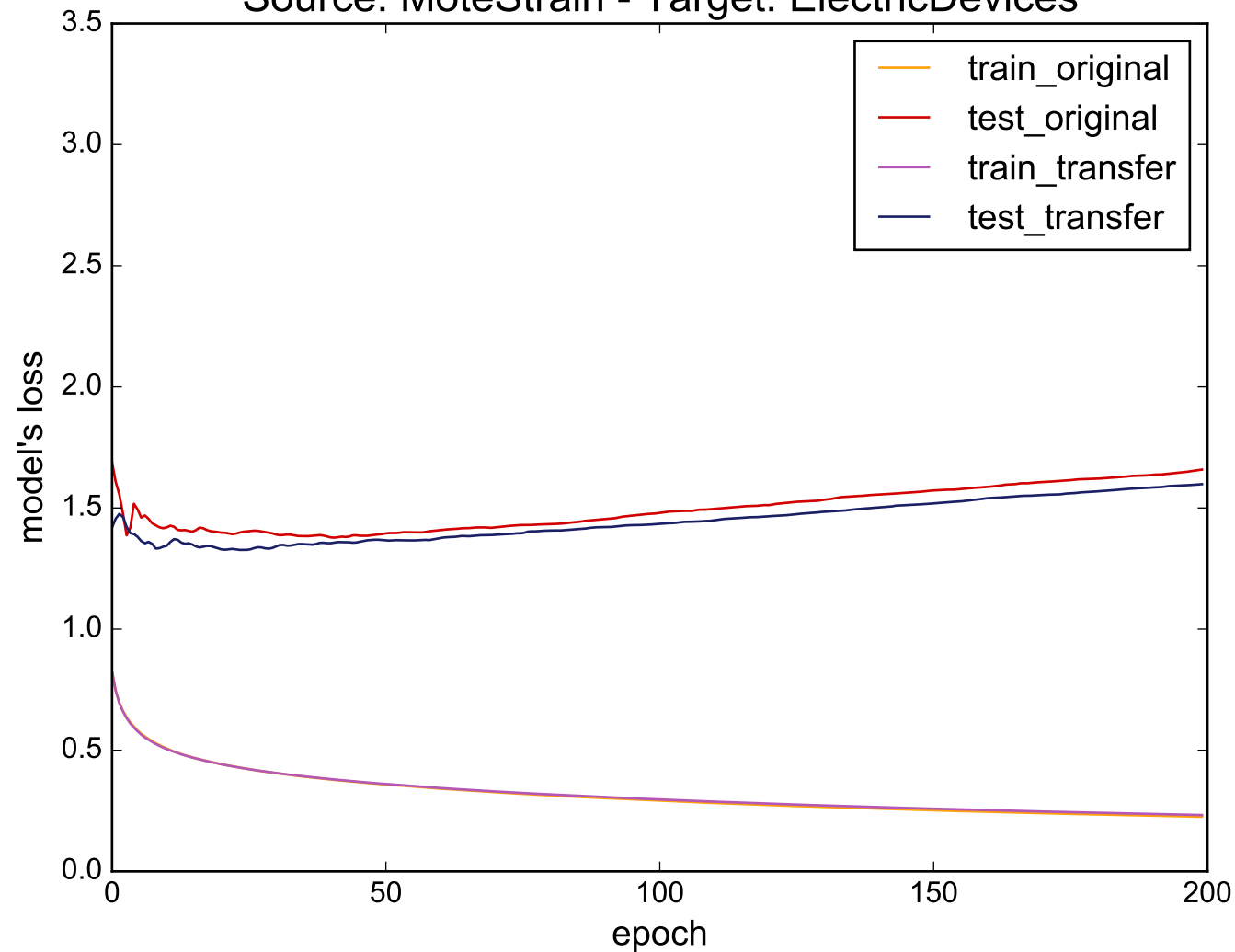
Source: MoteStrain - Target: ElectricDevices
