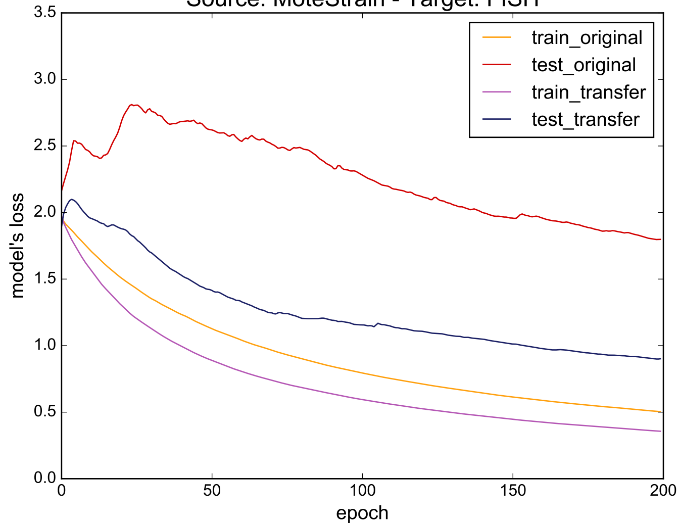
Source: MoteStrain - Target: FISH
