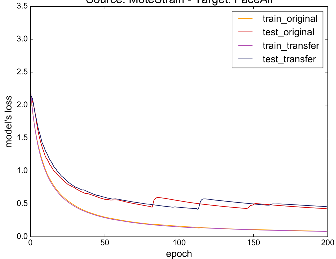
Source: MoteStrain - Target: FaceAll
