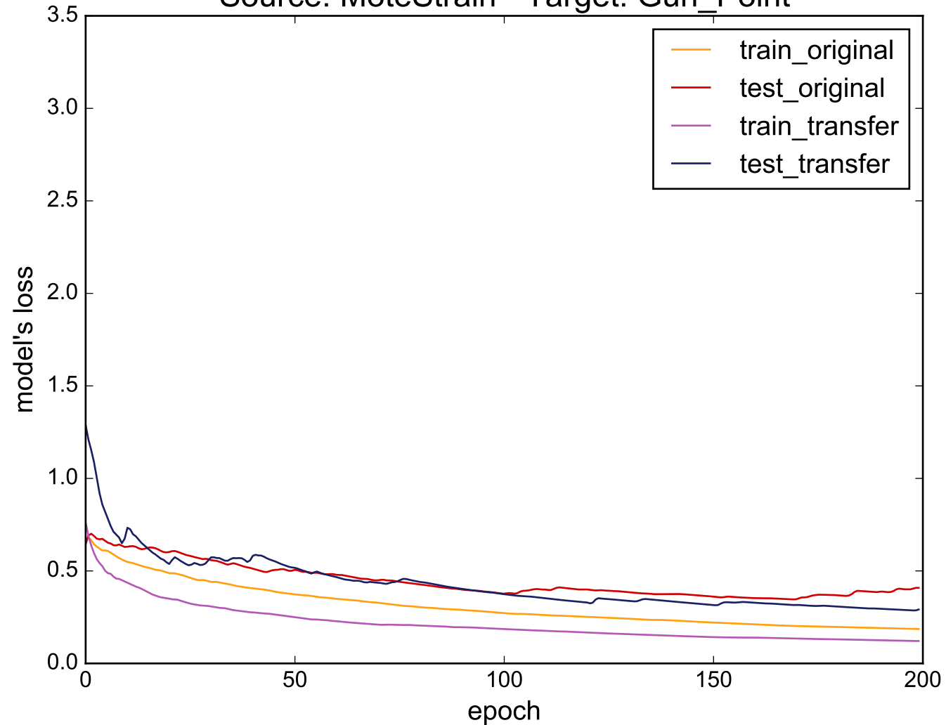
Source: MoteStrain - Target: Gun_Point
