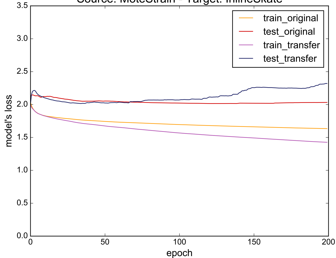
Source: MoteStrain - Target: InlineSkate
