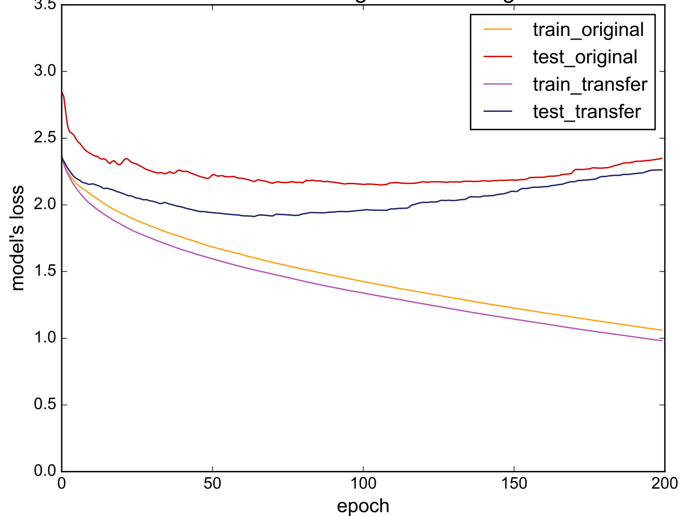
Source: MoteStrain - Target: InsectWingbeatSound
