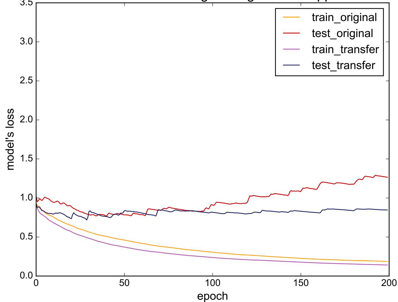
Source: MoteStrain - Target: LargeKitchenAppliances
