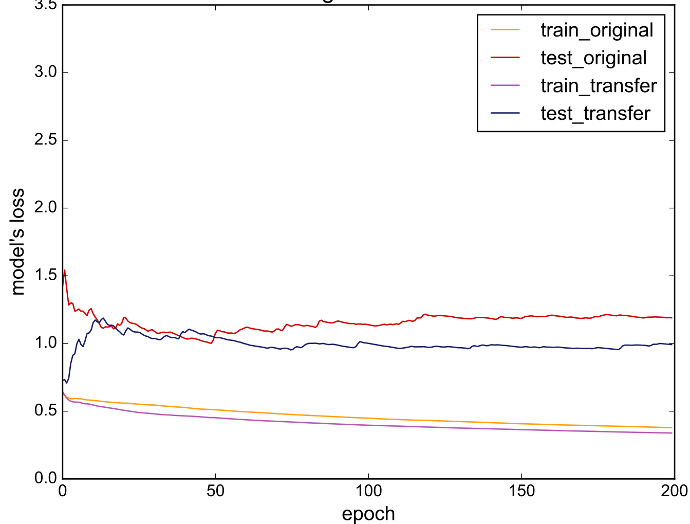
Source: MoteStrain - Target: MiddlePhalanxOutlineCorrect
