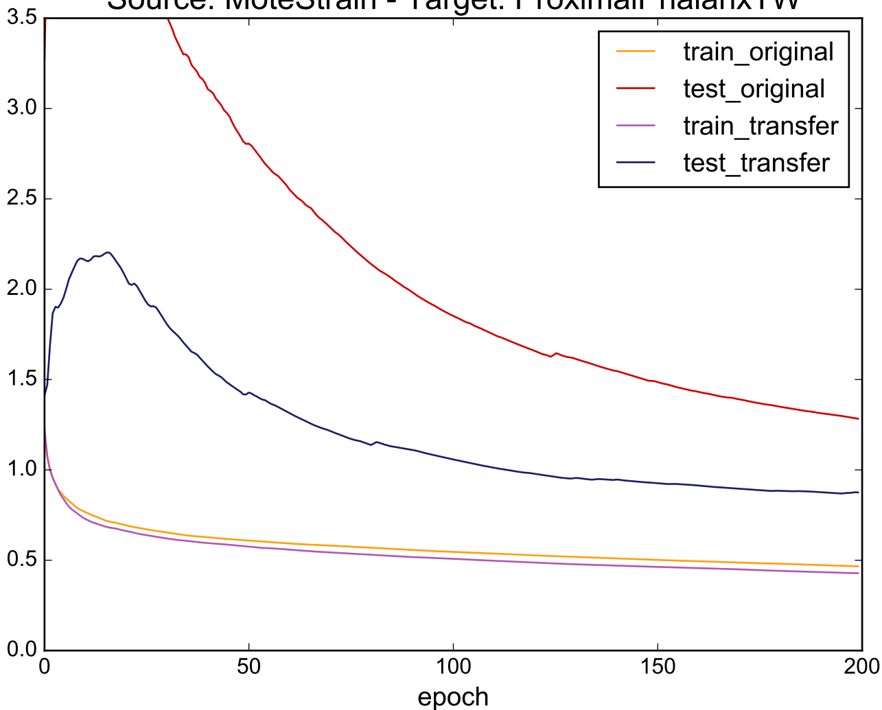
Source: MoteStrain - Target: ProximalPhalanxTW
