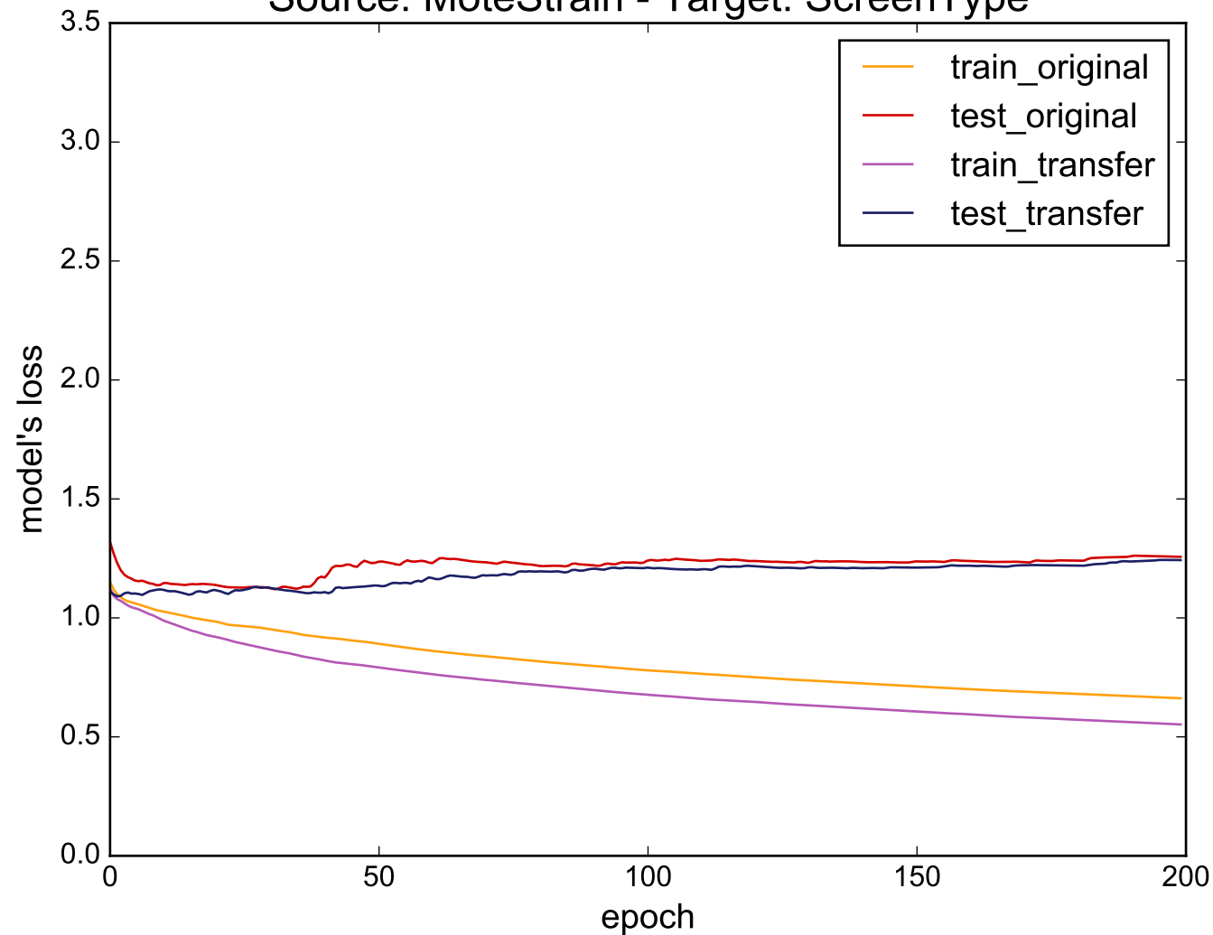
Source: MoteStrain - Target: ScreenType
