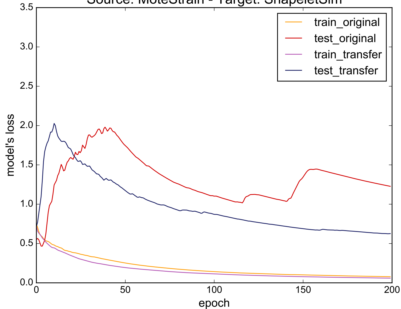
Source: MoteStrain - Target: ShapeletSim
