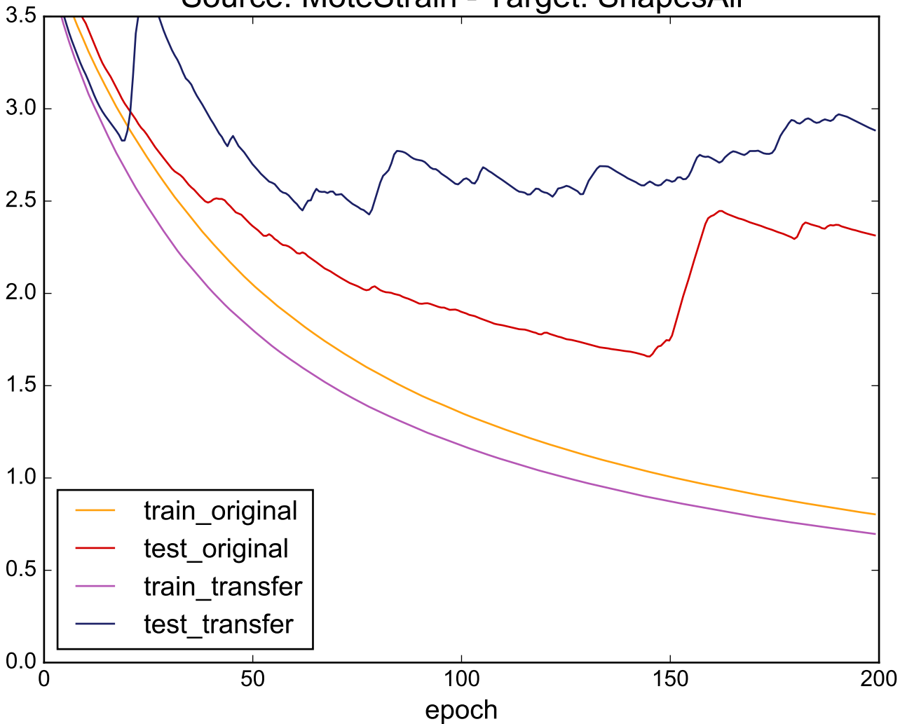
Source: MoteStrain - Target: ShapesAll
