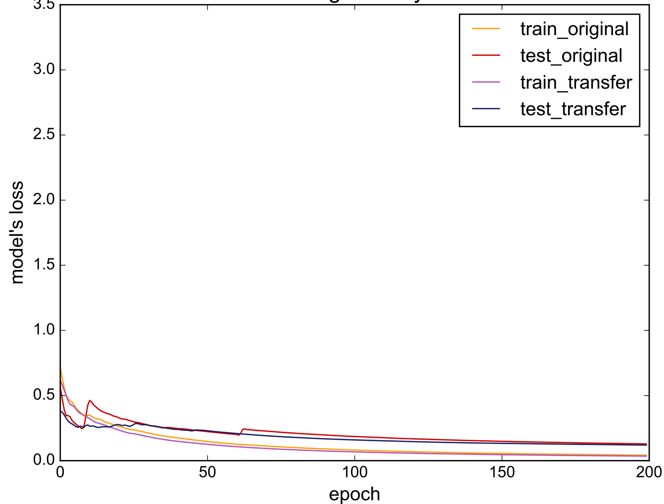
Source: MoteStrain - Target: SonyAIBORobotSurfacell
