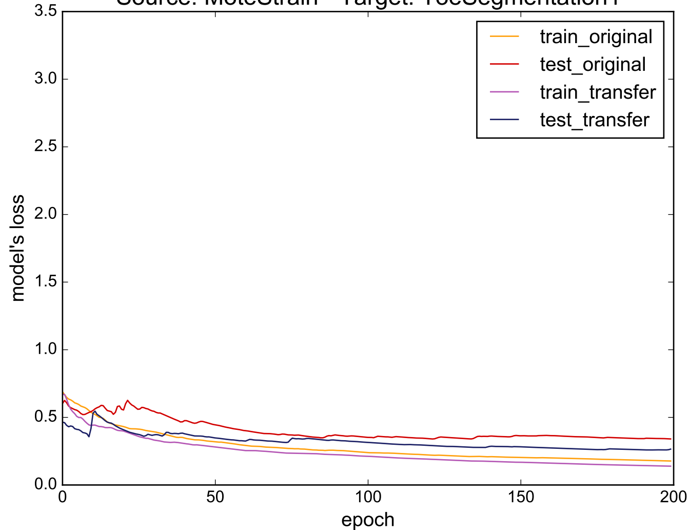
Source: MoteStrain - Target: ToeSegmentation1
