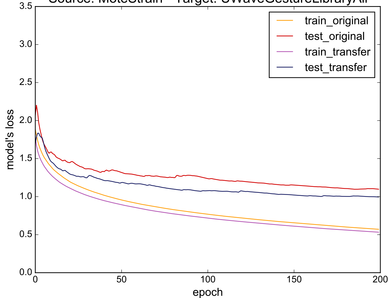
Source: MoteStrain - Target: UWaveGestureLibraryAll
