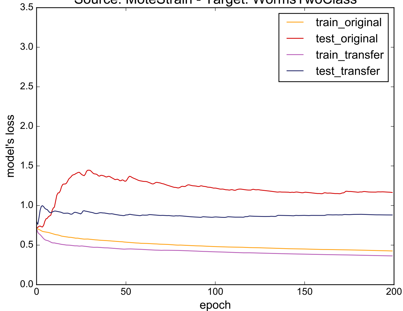
Source: MoteStrain - Target: WormsTwoClass
