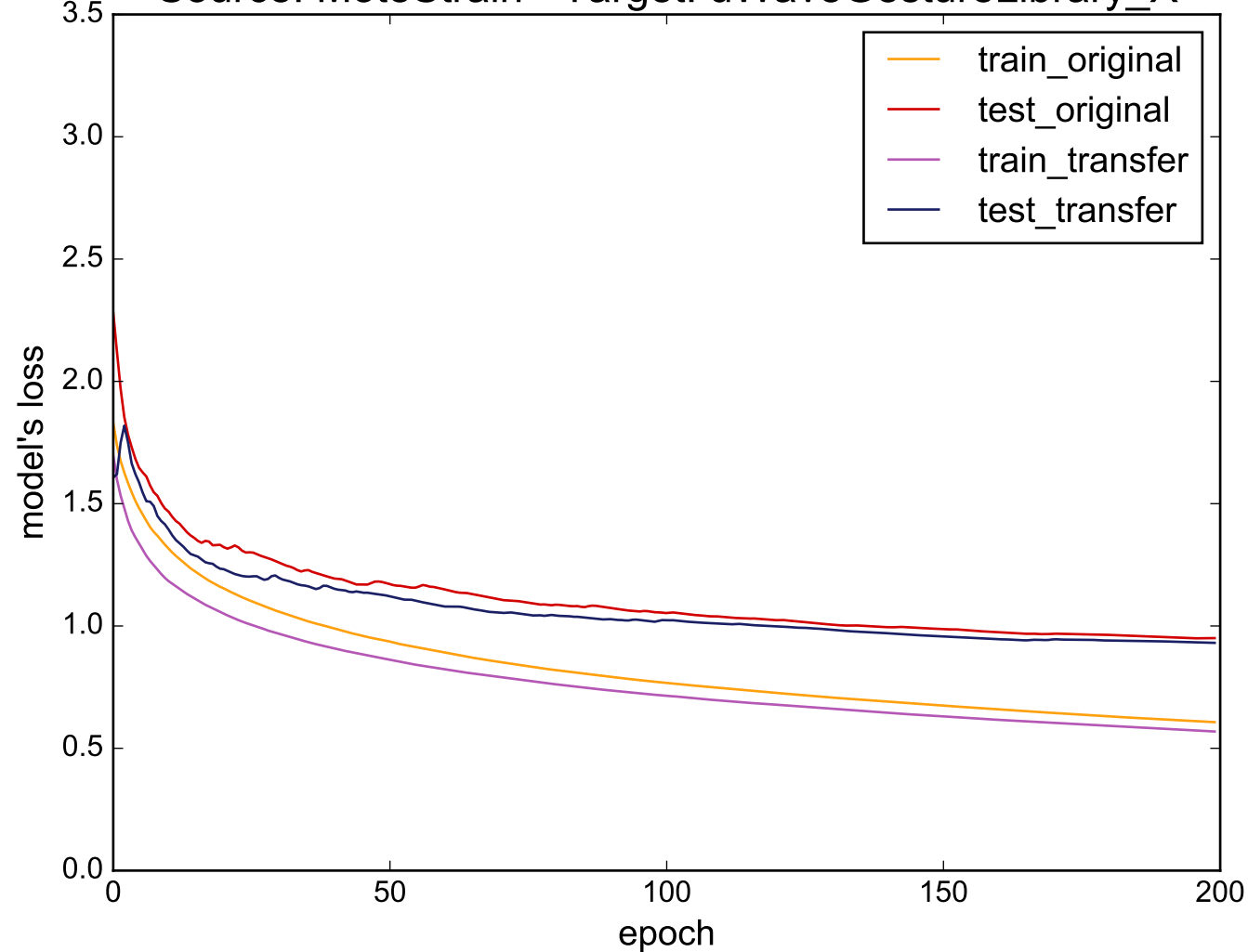
Source: MoteStrain - Target: uWaveGestureLibrary_X
