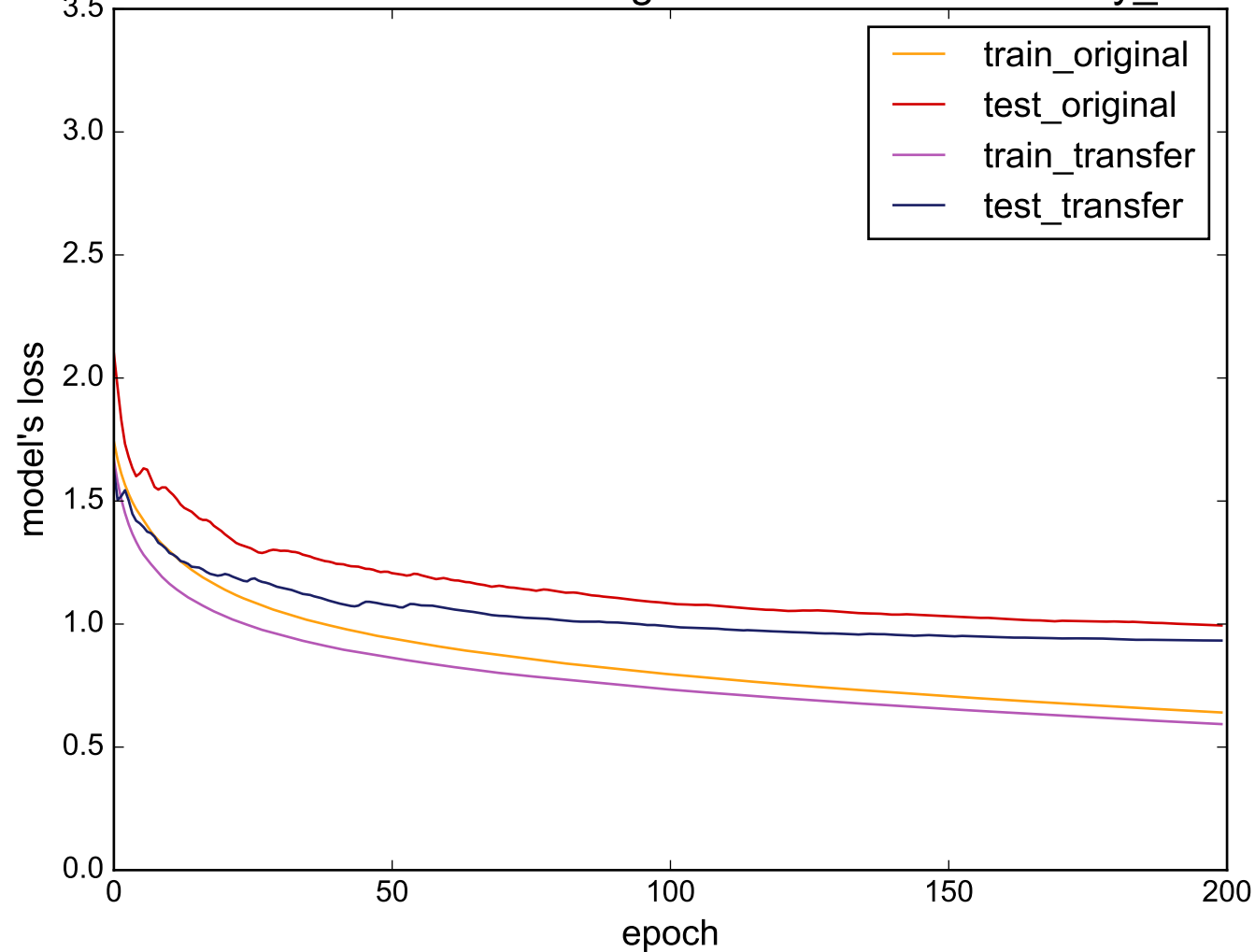
Source: MoteStrain - Target: uWaveGestureLibrary_Z
