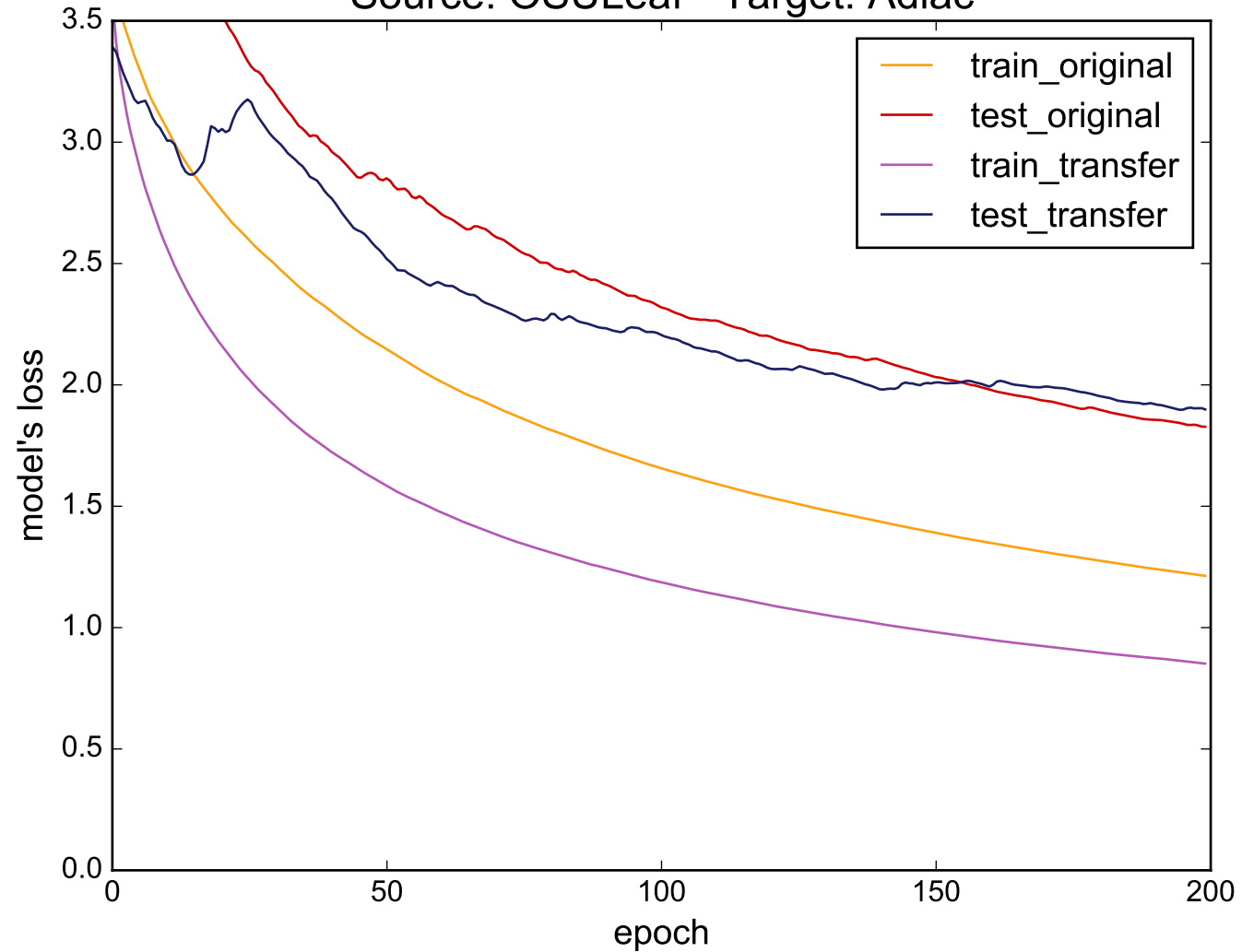
Source: OSULeaf - Target: Adiac
